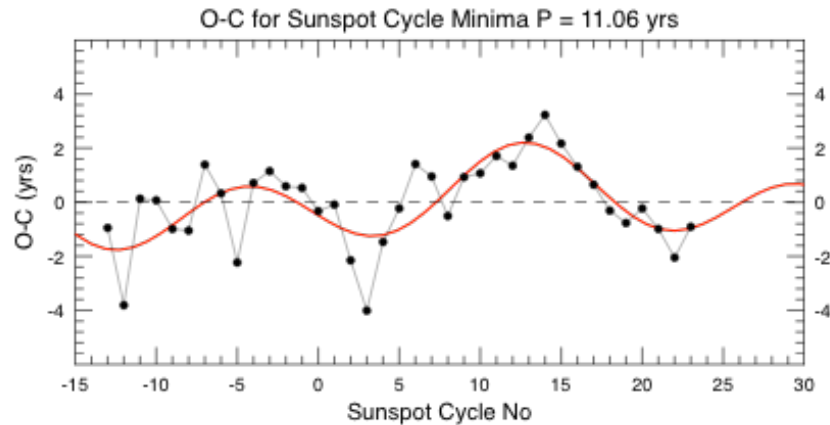
Figure 6: O-C for SCL minima compared with the dominating periods 190 and 440 years.
