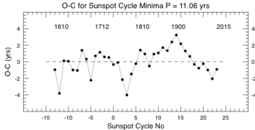
Figure 4: O-C residuals for the length of the solar cycle compared with the average period of 11.06 years. The curve is increasing for SCL > 11.06 yrs.
