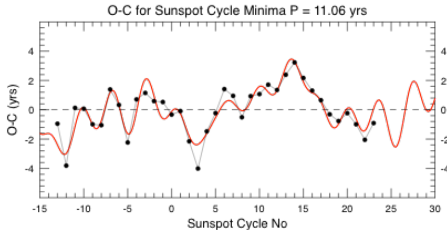
Figure 7: O-C residuals for SCL between minima, with a simulation based on 6 harmonics ( P = 440, 190, 86, 48, 43, \text{ and } 38 \text{ years} ).
