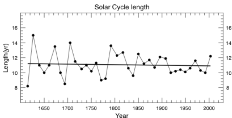
Figure 1: The Solar Cycle length from 1610 as downloaded from National Geophysical Data Center (NGDC). We observe that the SCL was longer than the mean of 11.06 years in most of the 19 th Century and shorter than the mean in most in the 20 th Century.
