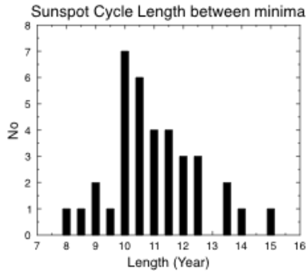
Figure 2: The distribution of the solar cycle length in bins of 0.5 years width. The distribution covers 36 cycles from 1610 to 2008.
