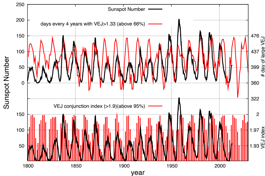
Figure 5. (Top) The sunspot number record (black) is compared against the number of days (every 4 yr) (red) when the alignment index IVEJ > 66 %. (Bottom) The sunspot number record (black) is compared against the most aligned days with IVEJ > 95 % (red). For details see Hung (2007) and Scafetta (2012c).
