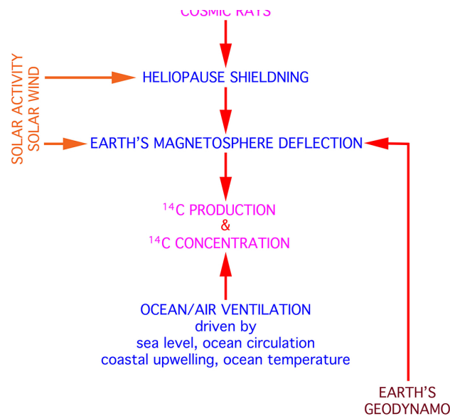
Figure 7. Illustration of the three factors controlling the ^{14}\text{C} production and concentration. Not until each factor is quantified, do we have a clear record of the solar variability.
