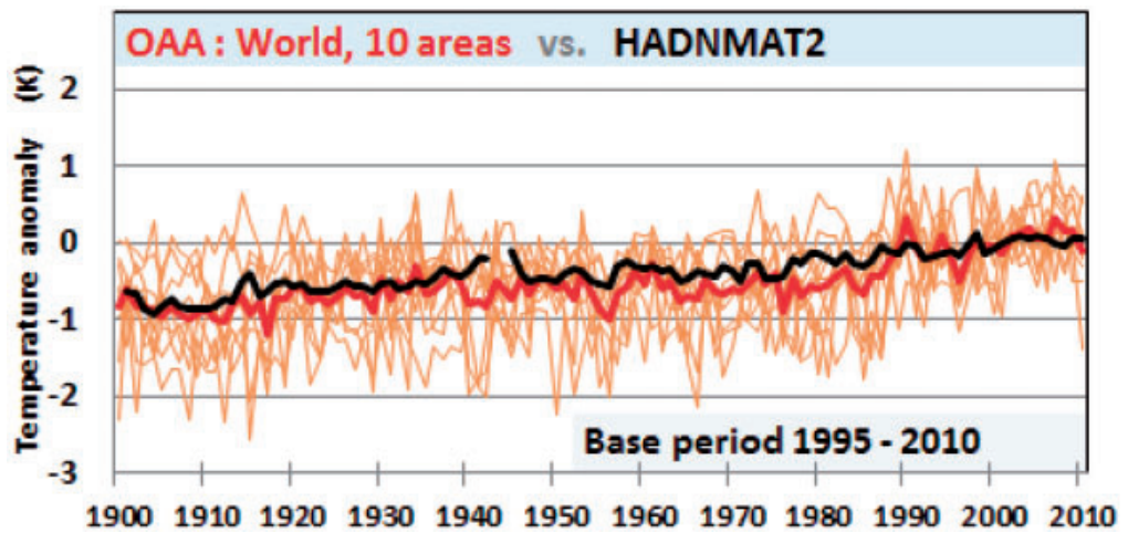
Figure 2. Sea surface temperature (HADNMAT2) compared with OA
