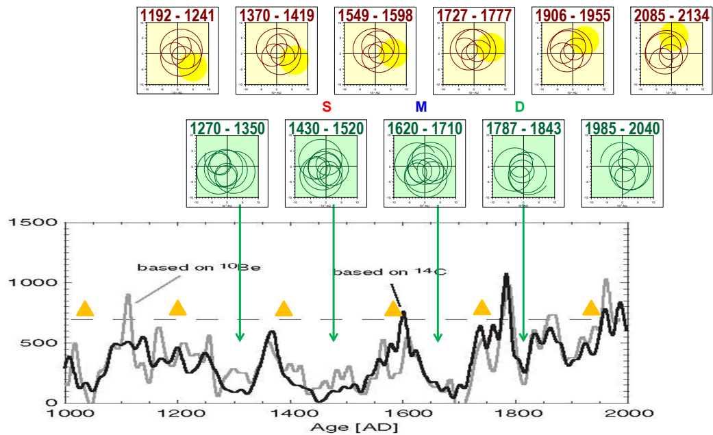
Figure 1: Above: the solar orbit divided into two basic types, the one ordered in JS (Jupiter/Saturn) trefoils (yellow) and one disorder (chaotic) (green). The Sun is returning at the trefoil orbits after 178.7 yr. The Sun moves in the area with a diameter of 4.3 r_s , where r_s is solar diameter or 3 \times 10^6 km. The yellow circles denote the Sun. Below: a solar modulation record based on ^{14}\text{C} and on ^{10}\text{Be} since 1000 AD (taken from Muscheler et al., 2007). Long-term maxima in these records tend to coincide with the trefoil intervals (yellow triangles mark their centres). Grand prolonged minima occurred in accordance with the intervals of the chaotic motion of the Sun (see lower green orbits), S – Spörer, M – Maunder, D – Dalton minima. A moderate chaotic (green) type of the SIM (1980–2040) indicates lowered both solar activity and surface air temperature.
