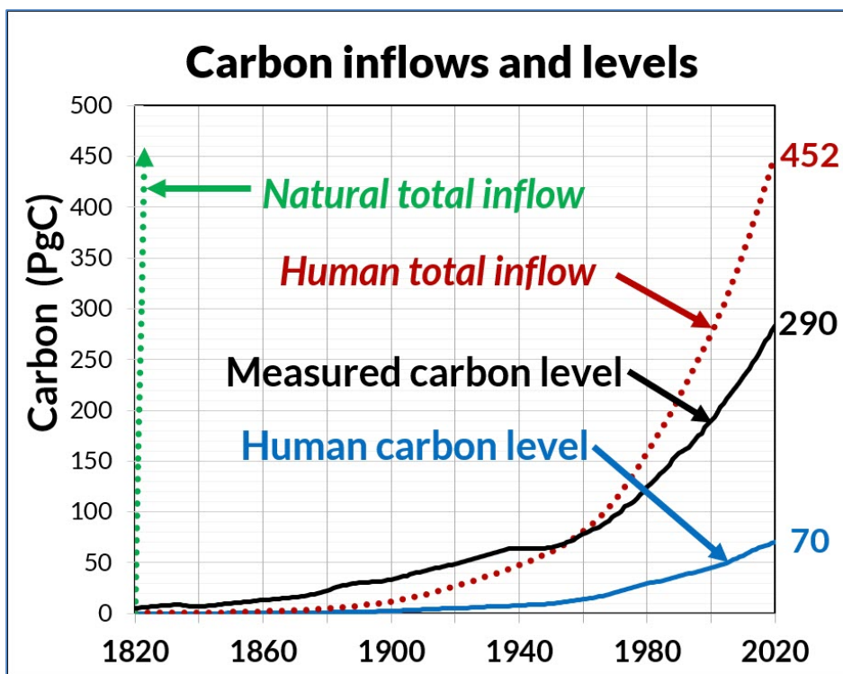
Figure 7. The blue line shows the human CO 2 level of IPCC's true human carbon cycle. The black line is the measured carbon level. The red dotted line is the accumulated human total carbon inflow since 1750 assuming all human emissions remained in the atmosphere. The green dotted line is the accumulated natural inflows.
